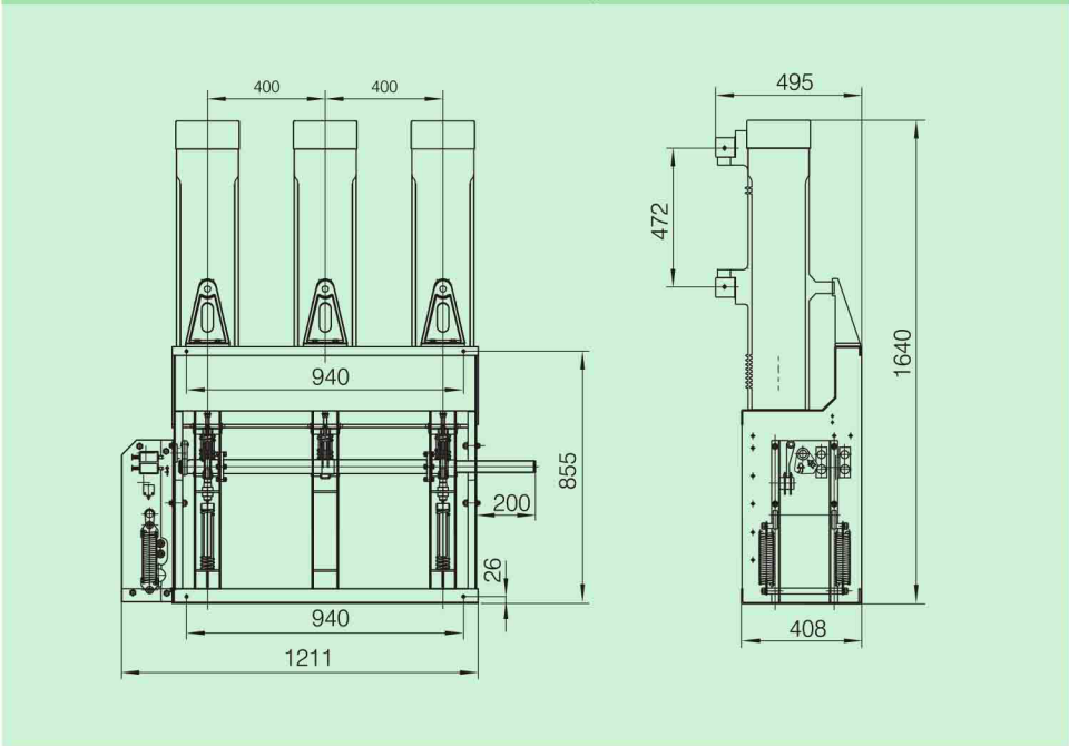
Fig.2 Side-mounted circuit breaker ZN85-40.5
